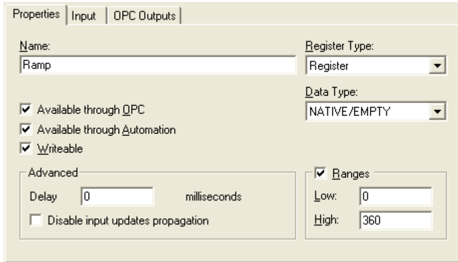
Figure 26: Properties
