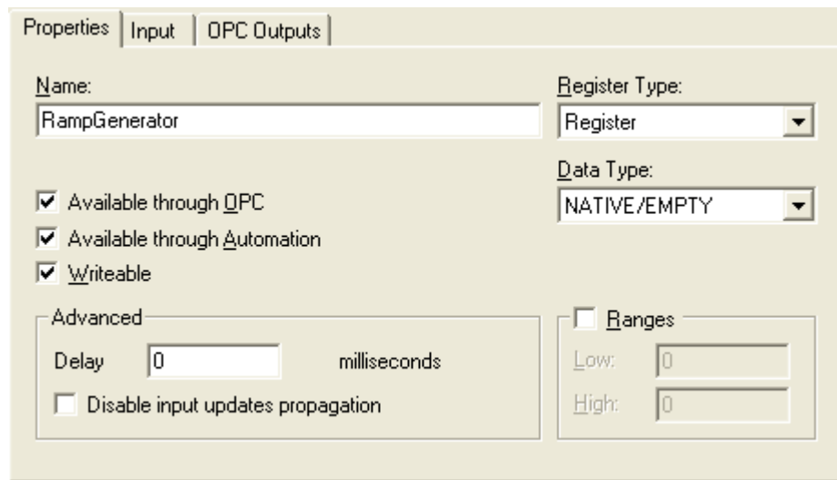
Figure 27: Properties
