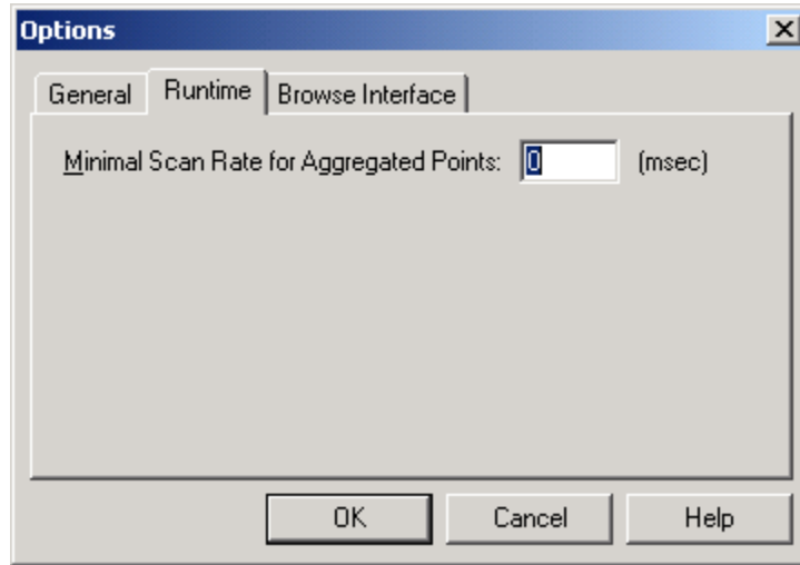
Figure 36: Runtime
