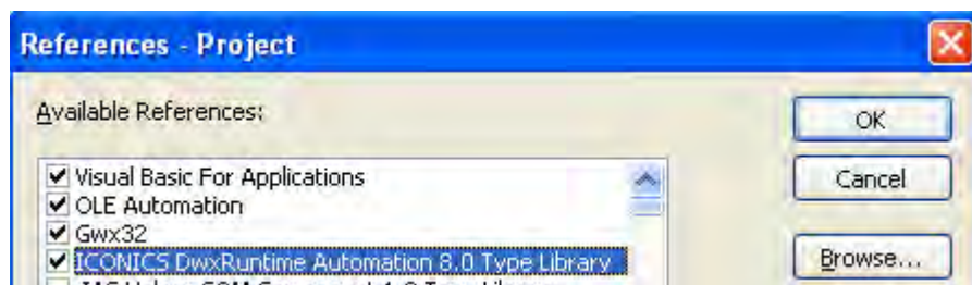
Figure 4: VBA References
