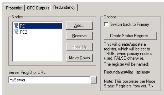
Figure 19: Redundancy Alias
