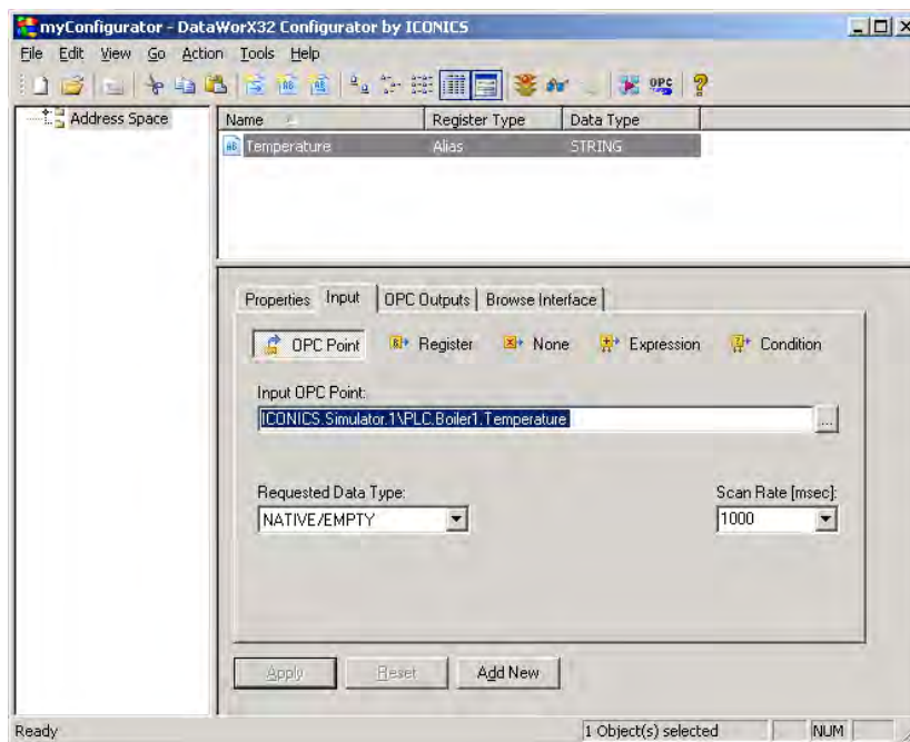
Figure 9: Alias Input
