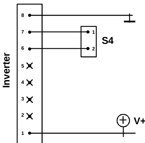
2) Dimming with variable analog DC voltage. Variable voltage 0 to 5 VDC (pin 7: 0 V)
