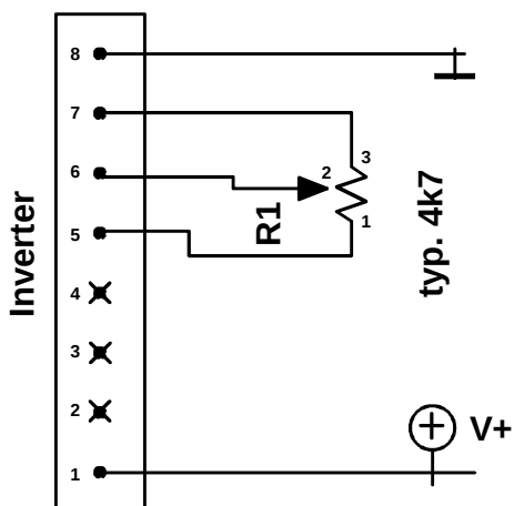
1) Dimming with variable Resistor (pin 7: 0 V)
