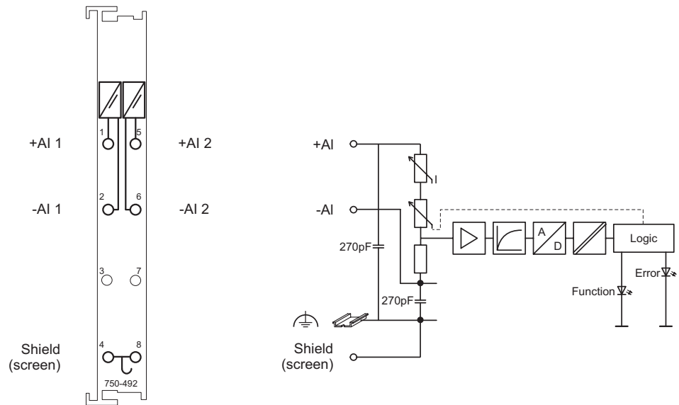
Fig. 2.1.1-3: 2-Channel Analog Input Module 4-20 mA
