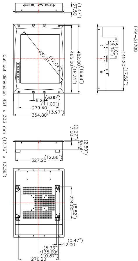
Figure 1.1: FPM-3171G Cutout Dimensions 451 x 333 mm (17.75" x 13.38")
