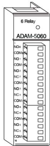
Figure 47: ADAM-5060 module frontal view
