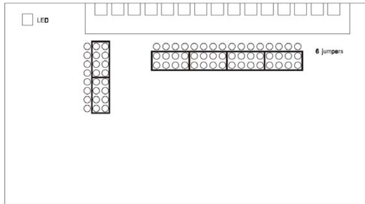
Figure 63: Jumper Location on the ADAM-5080 Module
