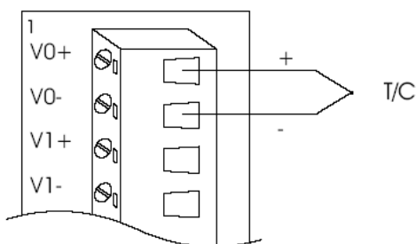
Figure 19: Thermocouple input
