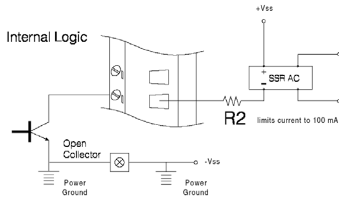
Figure 31: Digital output used with SSR (ADAM-5050/5056)
