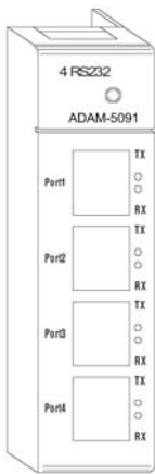
Figure 65: ADAM-5091 Module
