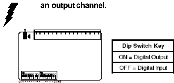
Figure 27: Dip switch setting for digital I/O channel
