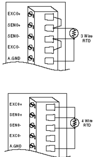
Figure 2: RTD inputs
