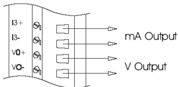
Figure 21: Analog output
