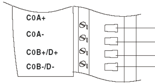
Figure 56: Wiring for Up/Down Counting
