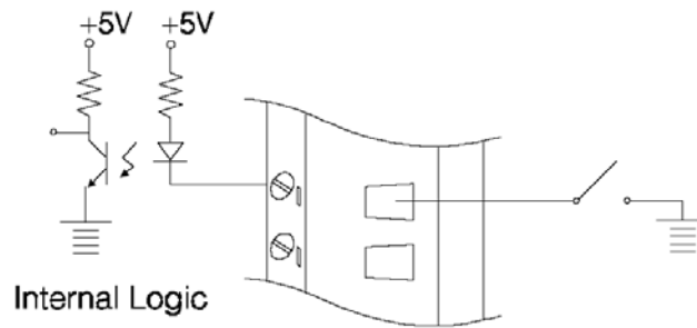
Figure 29: Dry contact signal input (ADAM-5050)
