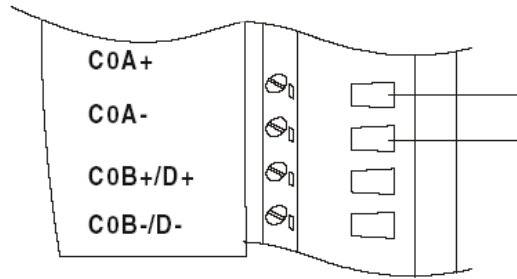
Figure 58: Wiring for Frequency Mode
